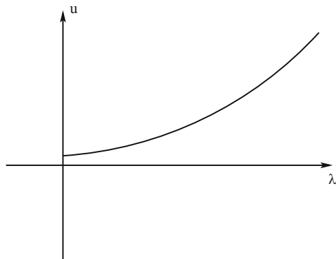
Fig. 4.1 The “sublinear” case m = 0
